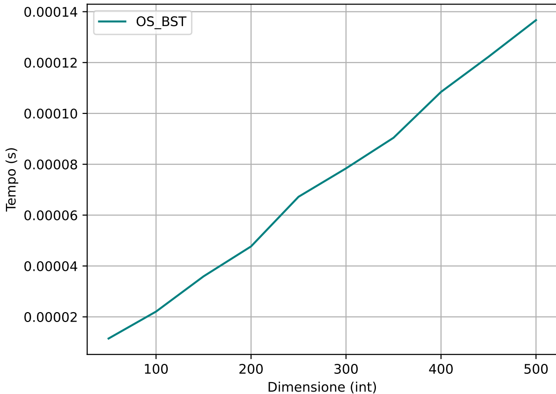
OS BST - Test Casual Deletion
